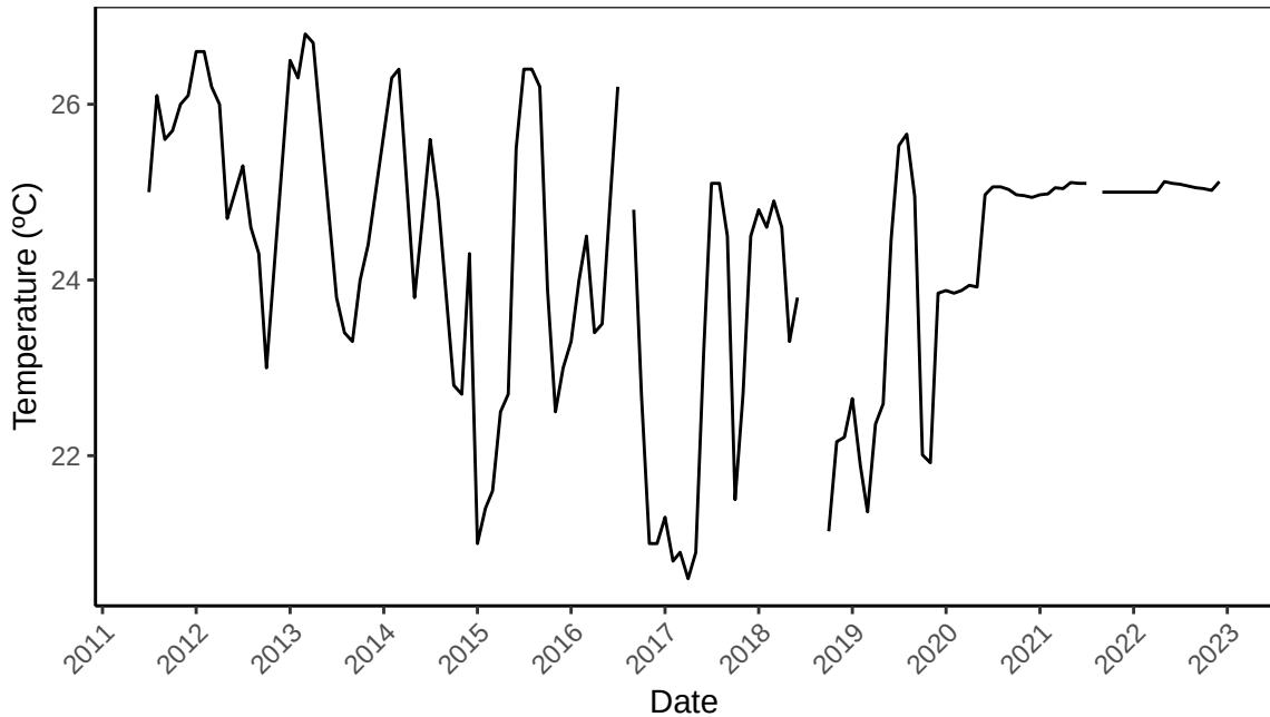
B2O Monthly Median Temperature (°C) from 2011–2023
