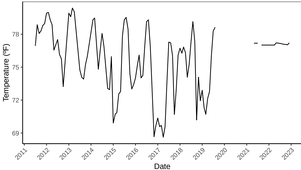
B2O Monthly Median Temperature (°F) from 2011–2023
