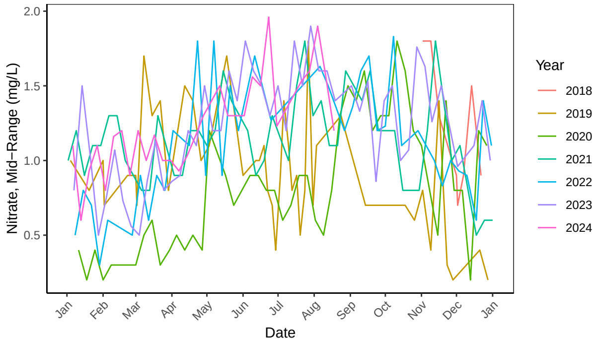
Biosphere 2 Mangroves Nitrate, Mid-Range (mg/L) from 2018–2024
