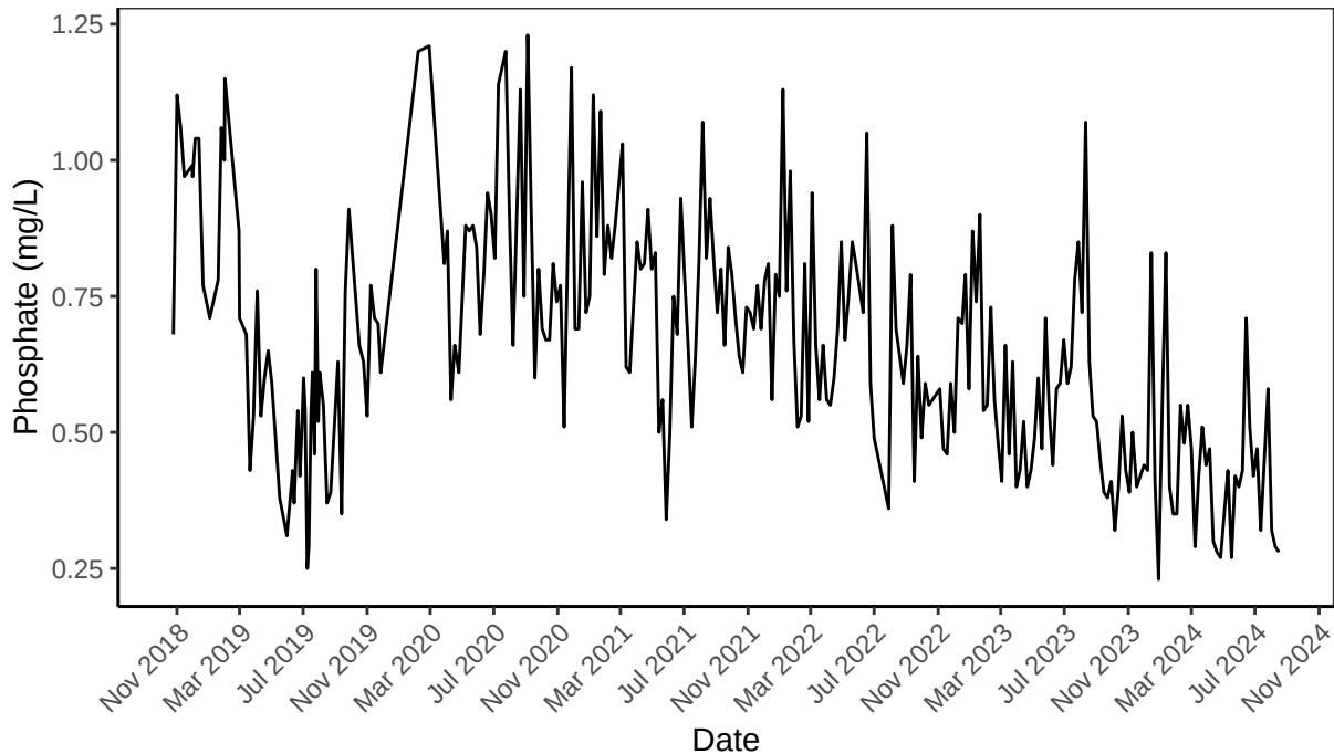
Biosphere 2 Mangroves Phosphate (mg/L) from 2018–2024
