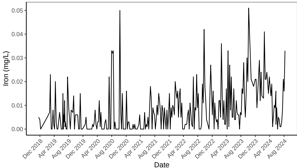
Biosphere 2 Ocean Iron (mg/L) from 2018–2024
