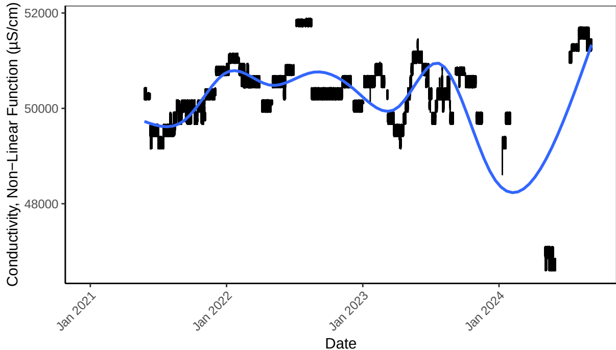
Conductivity, Non-Linear Function ( \mu\text{S}/\text{cm} )
