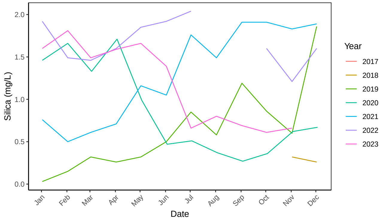
B2 Ocean Silica (mg/L) Monthly Median
