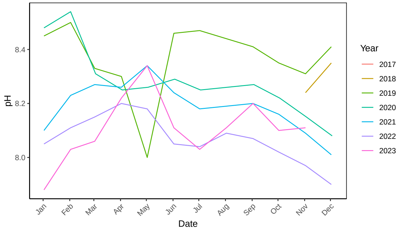
B2 Ocean pH Monthly Median
