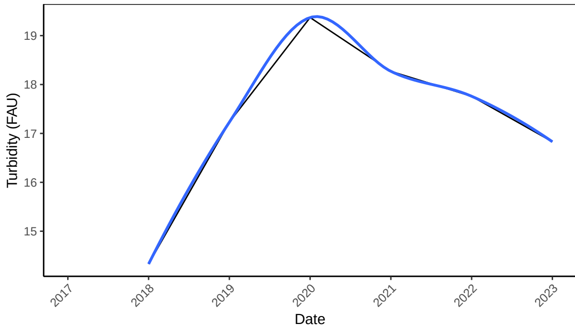
B2 Mangroves Turbidity (FAU) Yearly Mean
