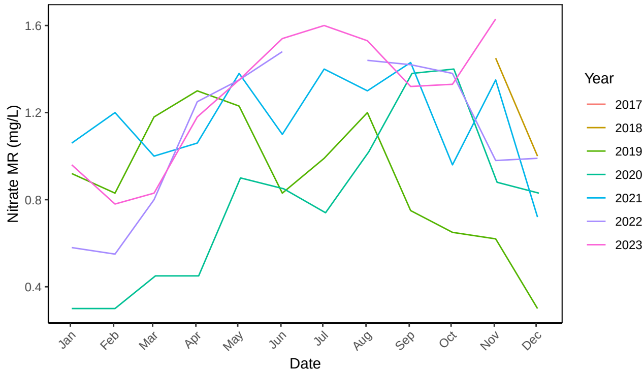
B2 Mangroves Nitrate MR (mg/L) Monthly Statistics
