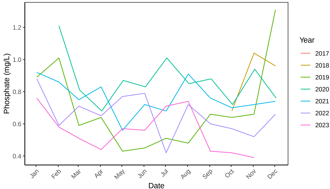
B2 Mangroves Phosphate (mg/L) Monthly Statistics
