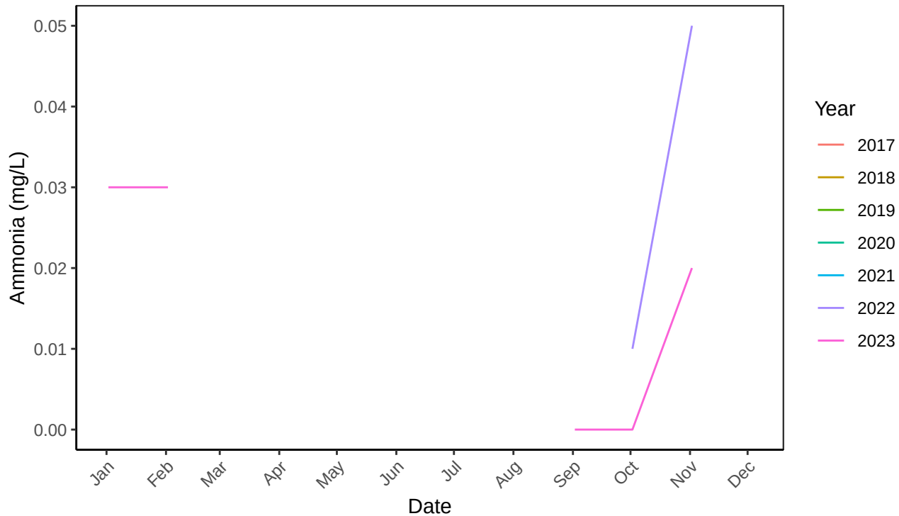
B2 Ocean Ammonia (mg/L) Monthly Statistics
