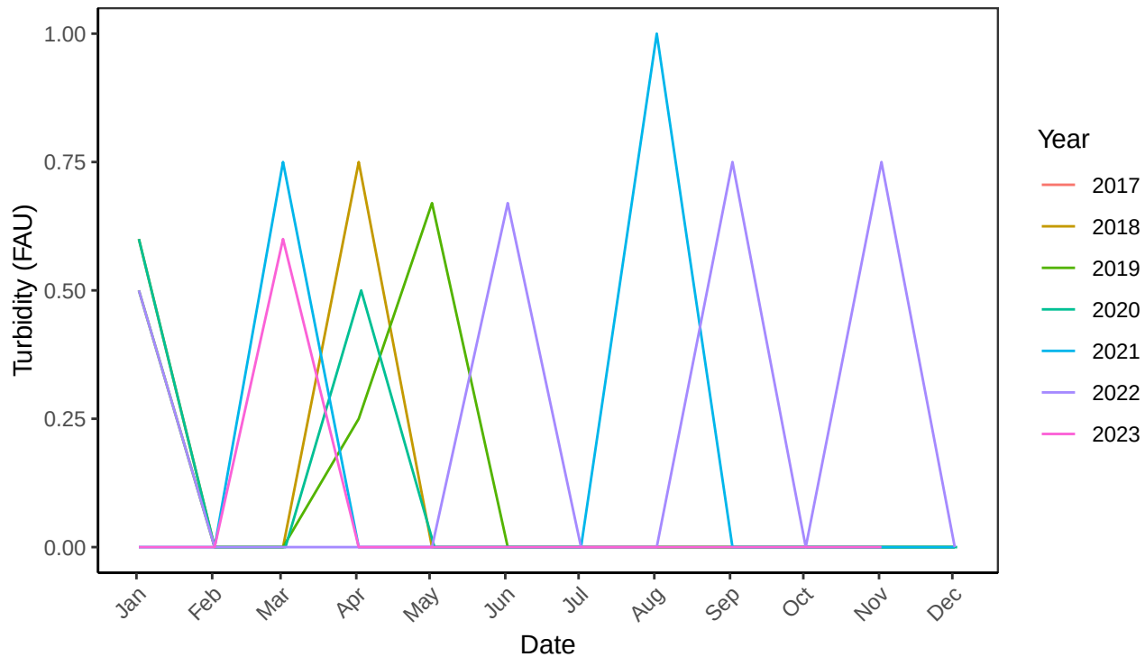
B2 Ocean Turbidity (FAU) Monthly Statistics
