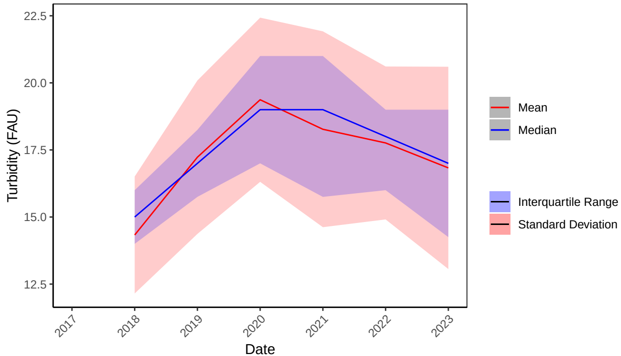
B2 Mangroves Turbidity (FAU) Yearly Statistics
