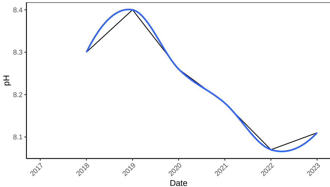
B2 Ocean pH Yearly Mean
