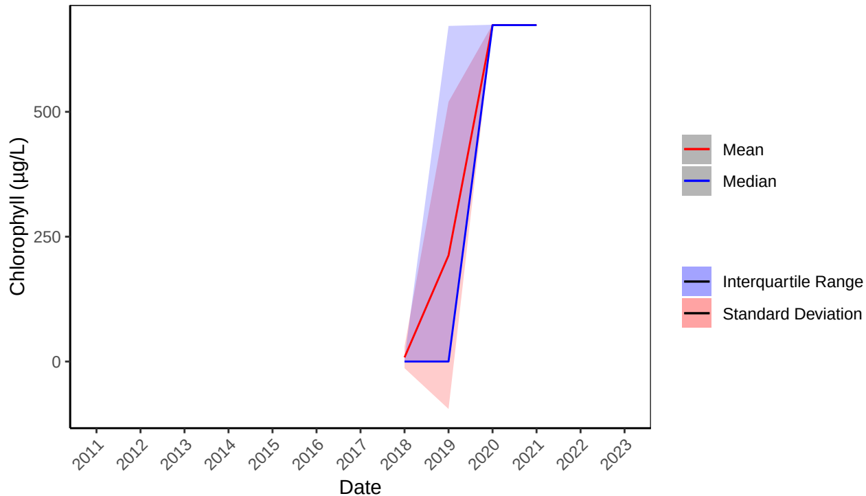
B2O Chlorophyll ( \mu\text{g/L} ) Yearly Statistics from 2011–2023
