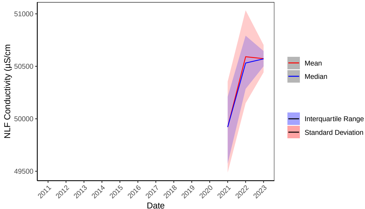
B2O NLF Conductivity ( \mu\text{S}/\text{cm} Yearly Statistics from 2011–2023
