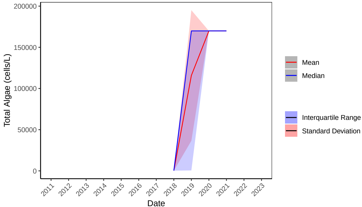
B2O Total Algae (cells/L) Yearly Statistics from 2011–2023
