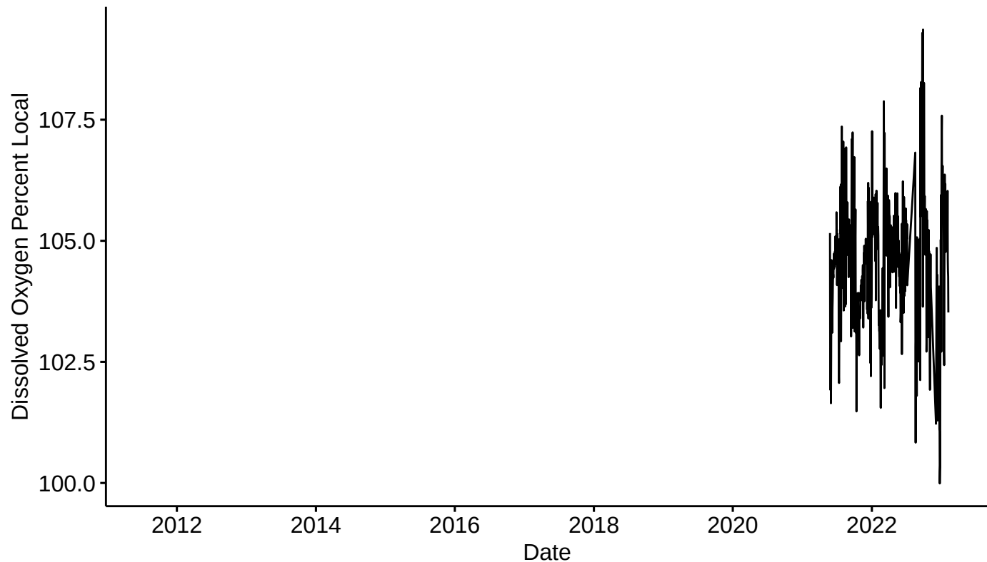
Post-QC B2O Dissolved Oxygen Percent Local Mean Daily Value from 2011
