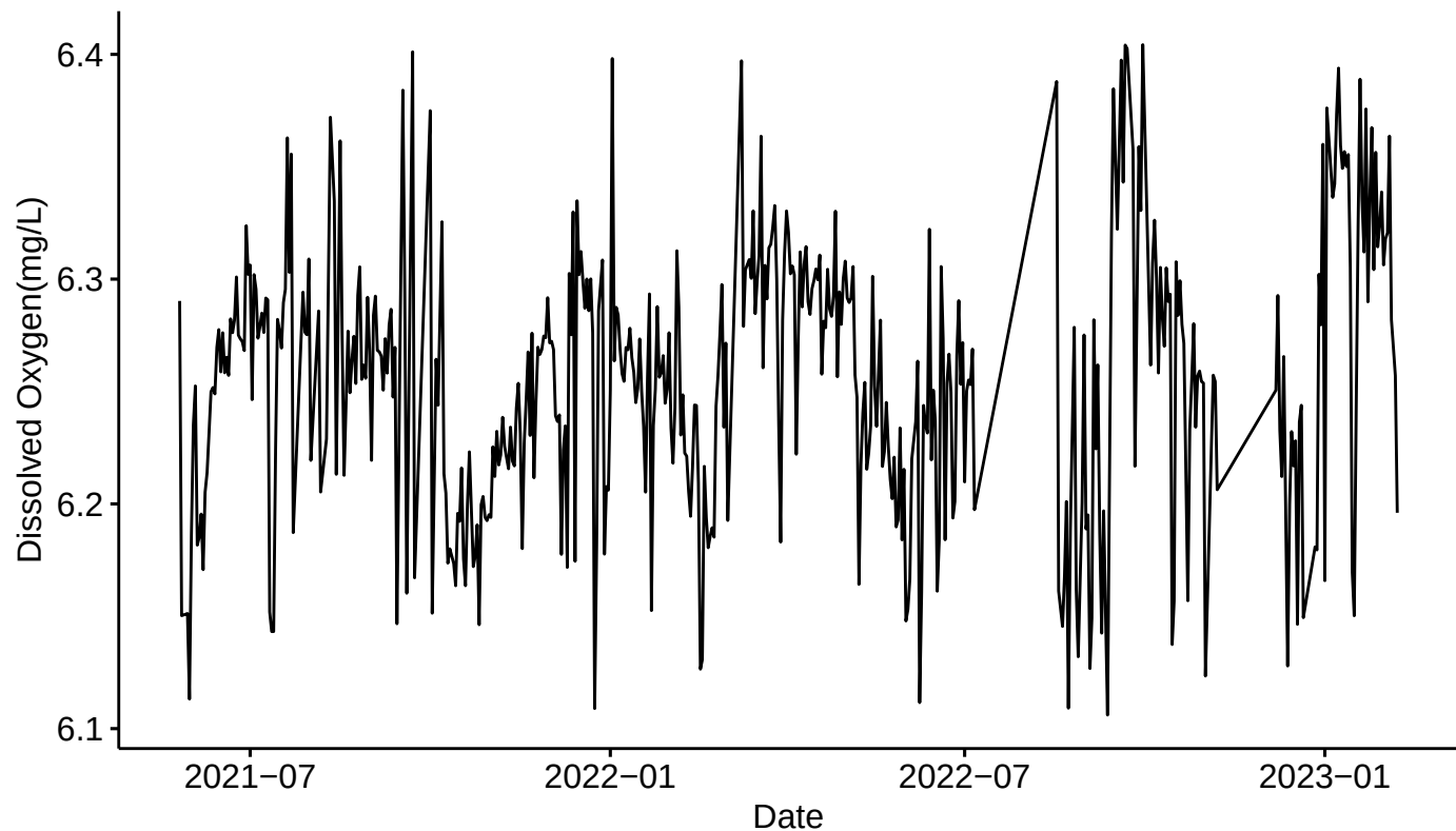
Post-QC B2O Dissolved Oxygen(mg/L) Mean Daily Value from 2021–2023
