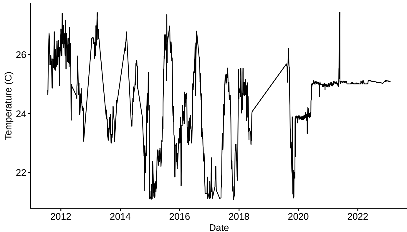
Post-QC B2O Temperature(C) Mean Daily Value from 2011–2023
