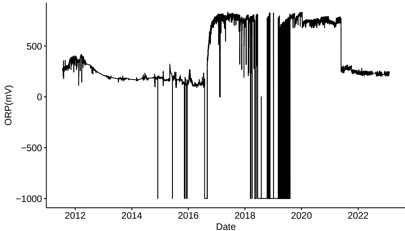
Pre-QC B2O Oxidation-Reduction Potential(mV) from 2011-2023
