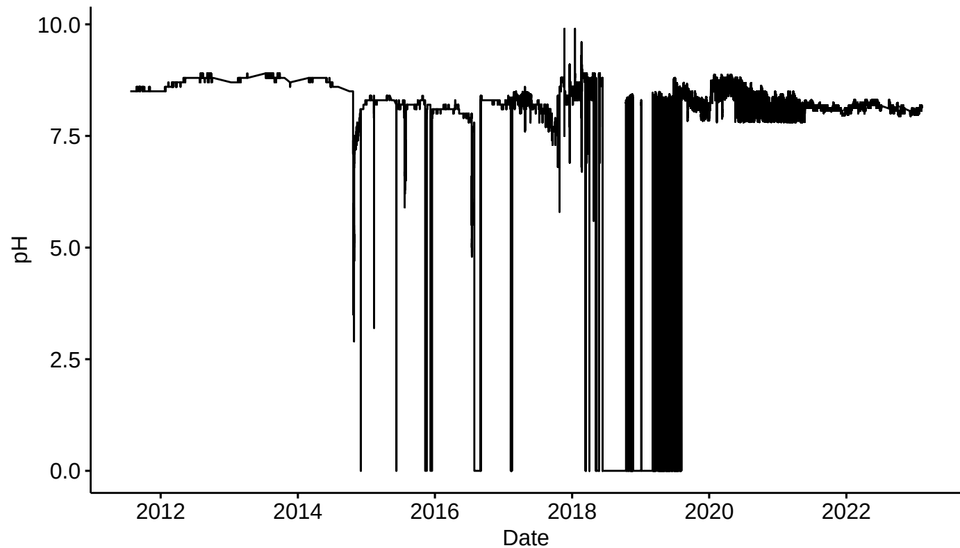
Pre-QC B2O pH from 2011–2023
