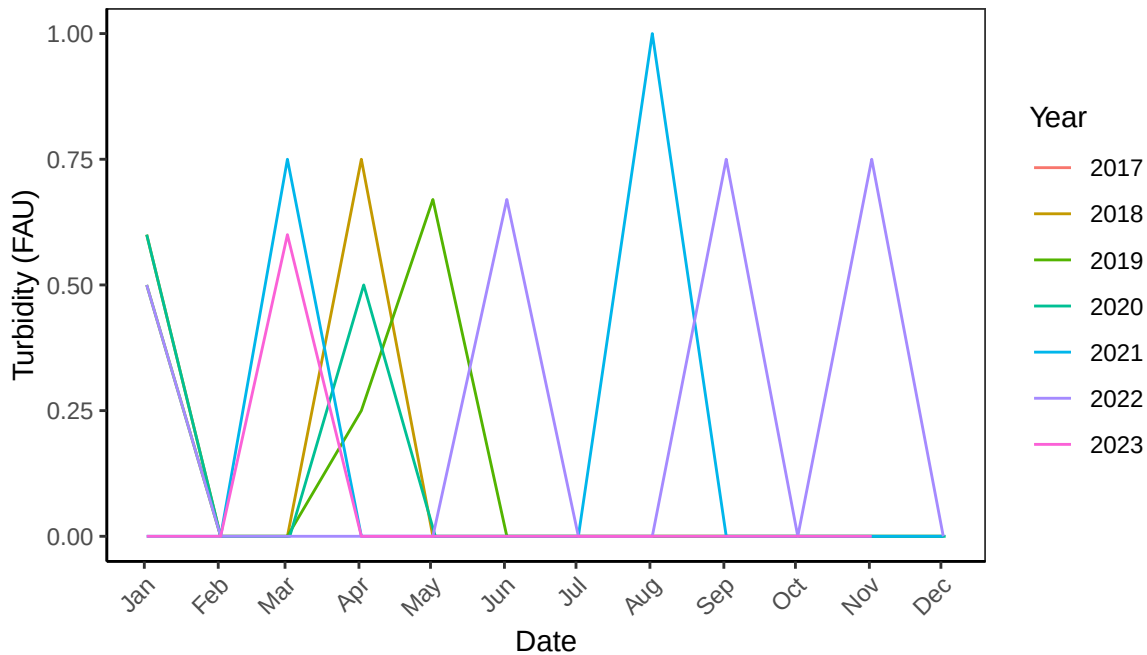
B2 Ocean Turbidity (FAU) Monthly Statistics
