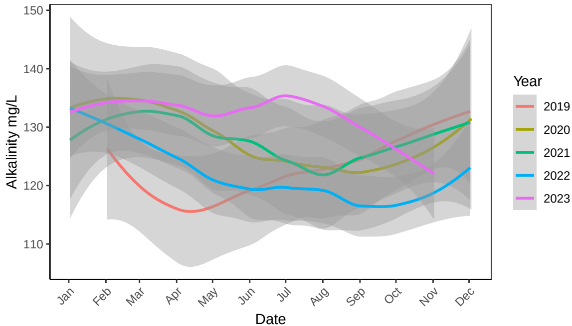
B2 Ocean Alkalinity mg/L Monthly Mean
