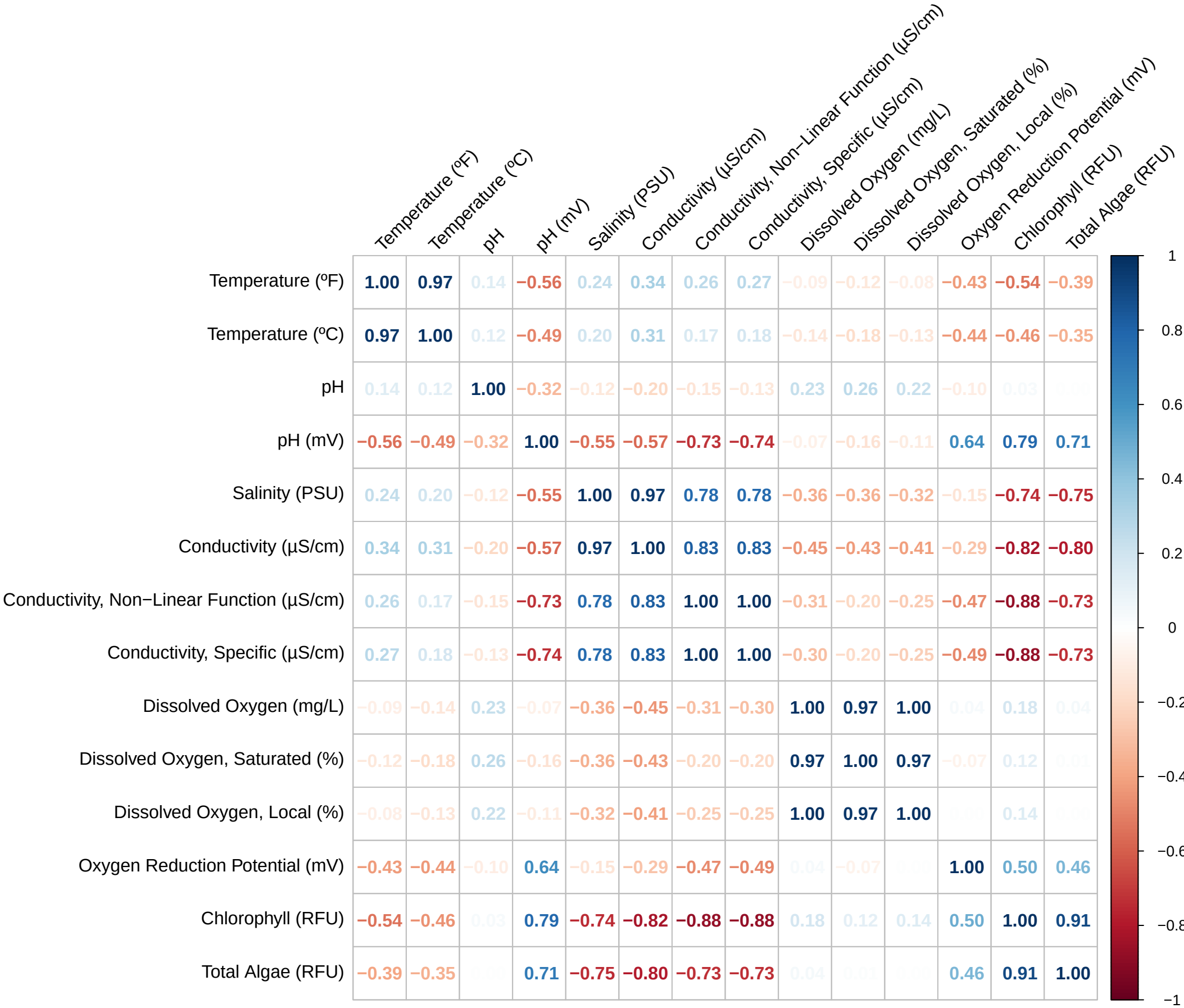
Biosphere 2 Ocean YSI Water Quality Correlations
