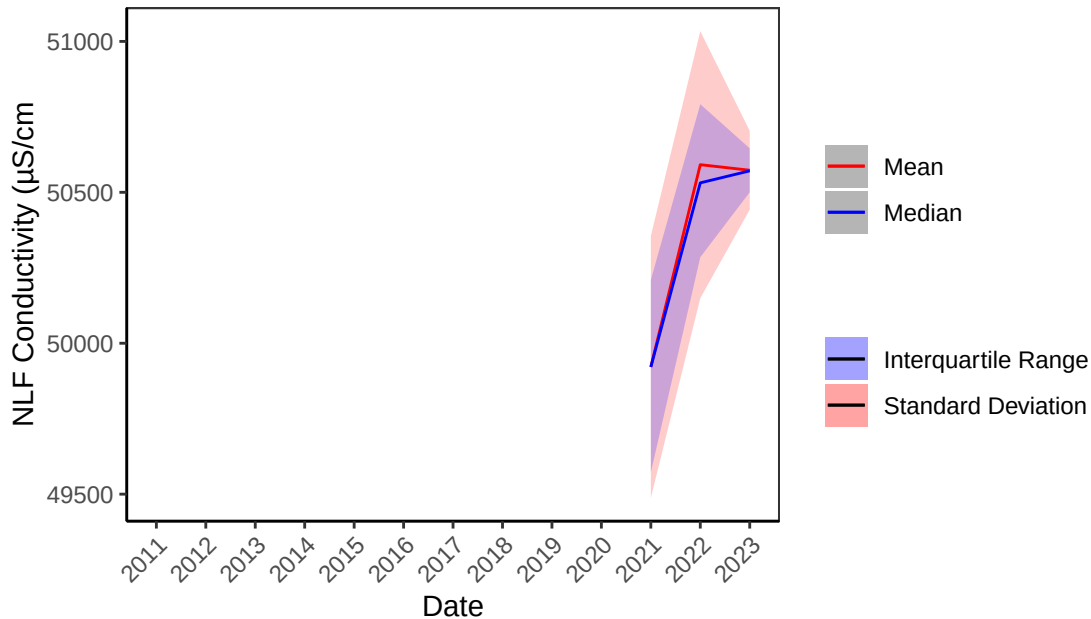
B2O NLF Conductivity ( \mu\text{S}/\text{cm} Yearly Statistics from 2011–2023
