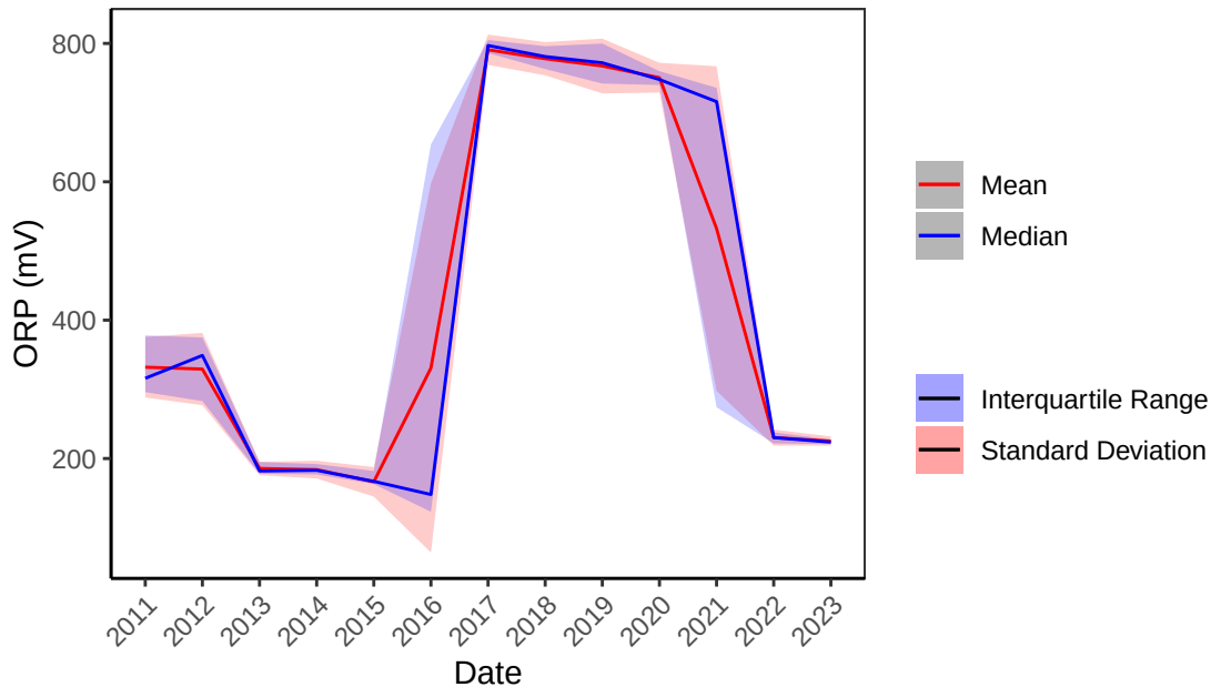
B2O ORP (mV) Yearly Statistics from 2011–2023
