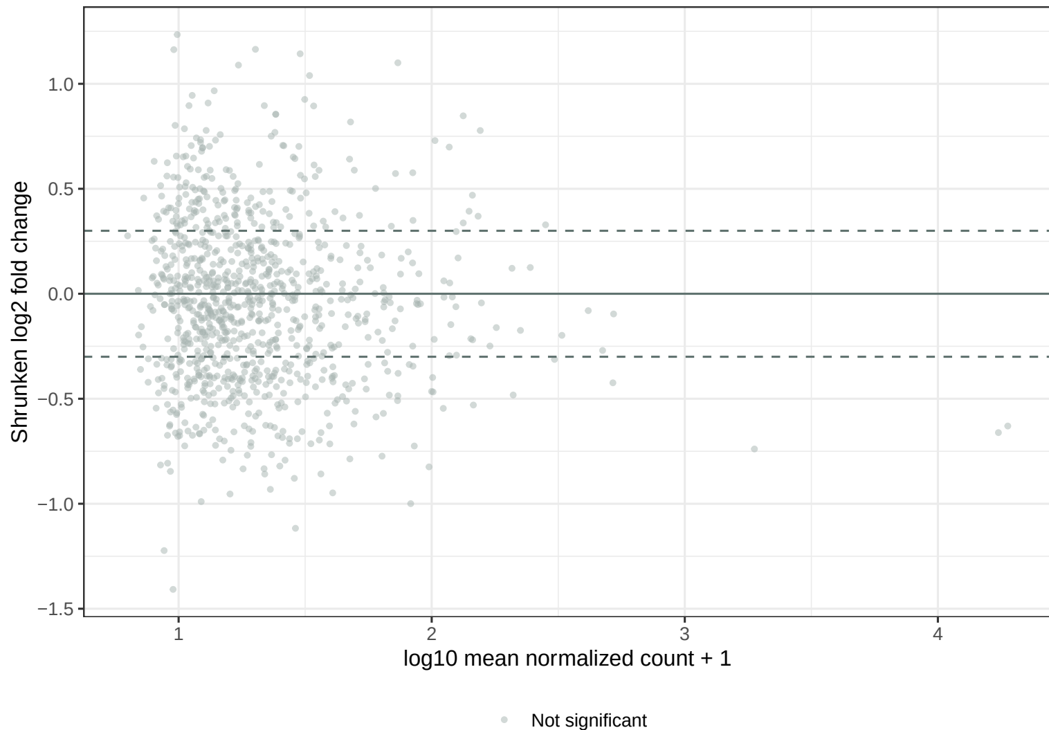
MA plot – lncRNA OD1 vs H
