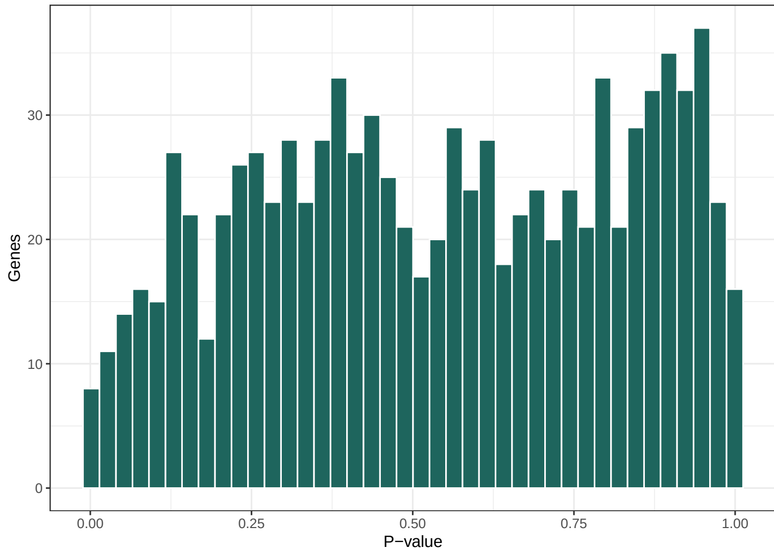
P-value distribution – lncRNA
