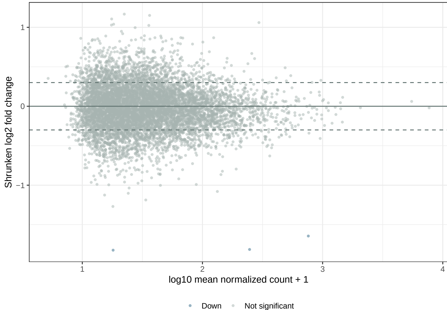
MA plot – mRNA OD1 vs H
