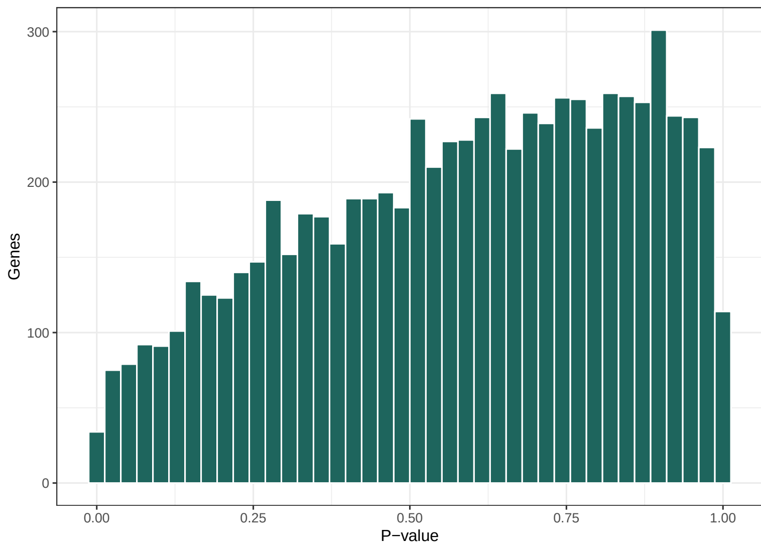
P-value distribution – mRNA
