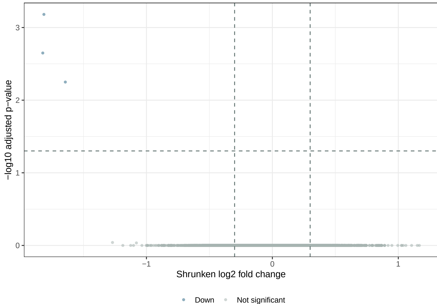
Volcano plot – mRNA OD1 vs H
