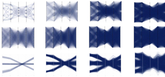
Fig. 9. The technique of progressive parallel coordinates [38].
