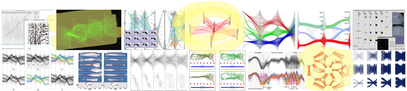
Fig. 1. Examples of extensions and modifications of parallel coordinates that have been evaluated. All images are reproduced with the permission of their respective copyright holder.
