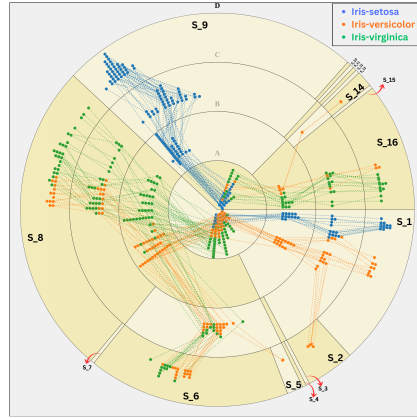
Fig. 3: Iris Dataset visualised in hierarchical rings and sectors using modified algorithm.
