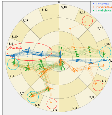
Fig. 4: Iris Dataset - RAYS Visualisation [Red Marking - Pure class; Blue Marking - Mixed Class]
