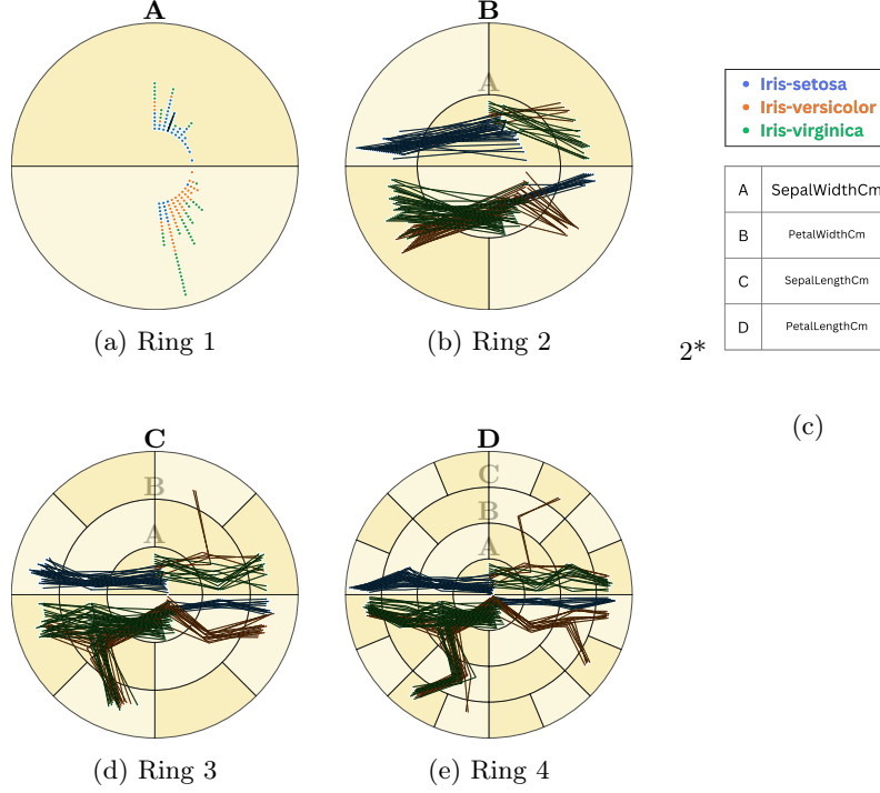
Fig. 2: Iterative ring construction and point placement (Iris Dataset)
