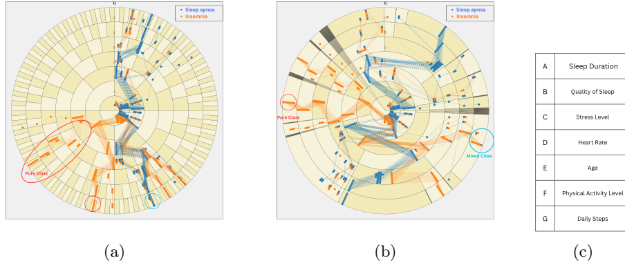
Fig. 5: Sleep-Lifestyle (7-dimensional) Dataset - RAYS Visualisation comparing (a) uniform sector partitioning and (b) proportional sector partitioning, with (c) the ring label legend.
