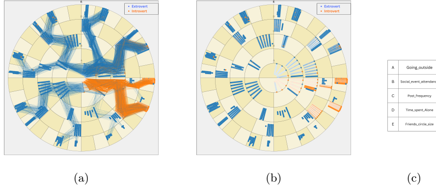
Fig. 6: Extrovert-Intervert Personality Survey Dataset (5-dimensional) - RAYS Visualisation comparing (a) uniform sector partitioning and (b) proportional sector partitioning, with (c) the ring label legend.
