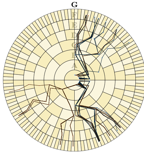
Fig. 5: Sleep-lifestyle (8-dimensional) Dataset with 2 labels - RAYS Visualisation
