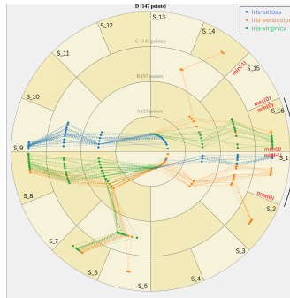
Fig. 3: Iris Dataset points plotted in hierarchical rings and sectors with marking of the scale used to plot the points in the sectors based on their values.
