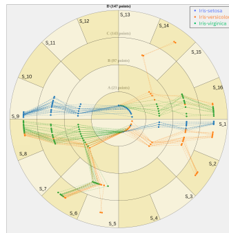
Fig. 1: Iris Dataset with 3 labels - RAYS Visualisation
