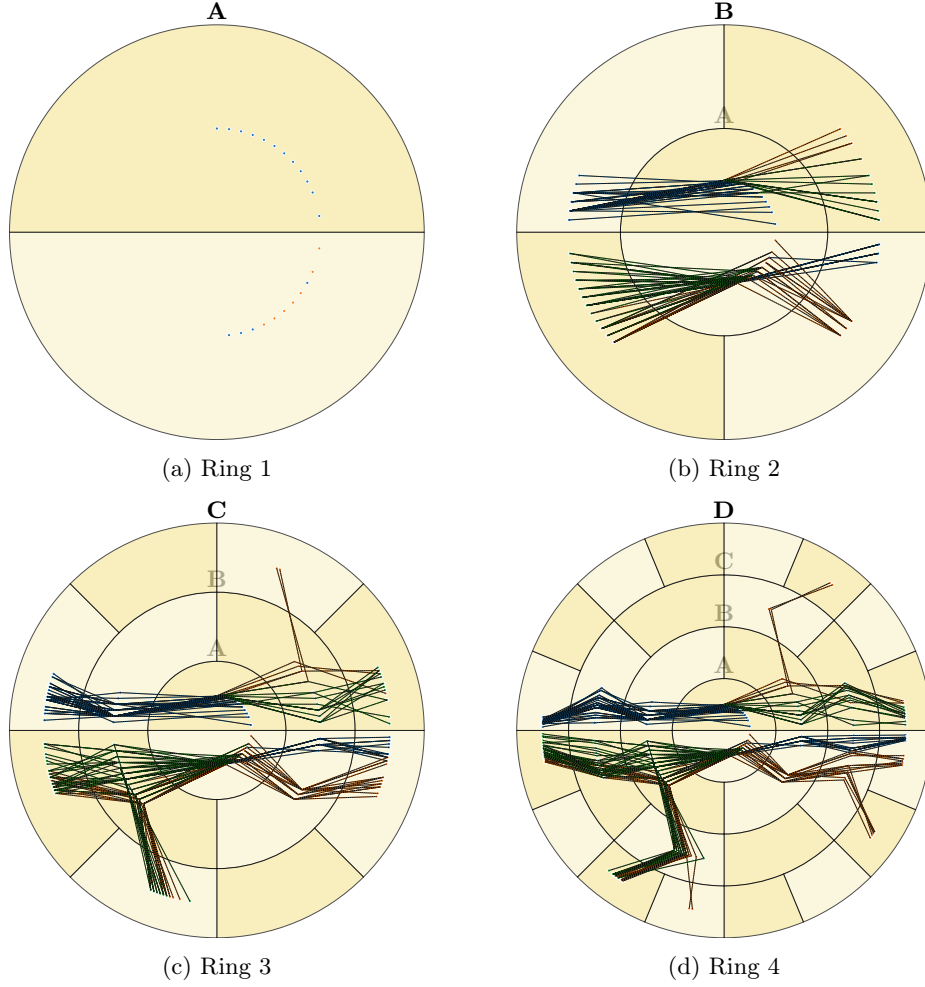
Fig. 2: Iterative plotting of points in rings/dimensions
