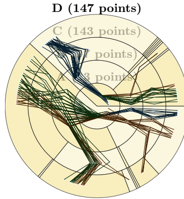
Fig. 4: Iris Dataset points plotted in hierarchical rings and sectors with the help of modified algorithm.
