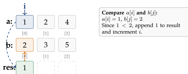
Figure: Two-pointer comparison: a[i] = 1 is smaller than b[j] = 2 , so it is appended to the result, and pointer i advances.
