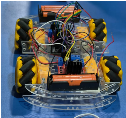
Figure 5.1: Assembled 4WD Robot Car
