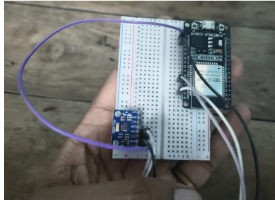
Figure 5.6: Transmitter View 1
