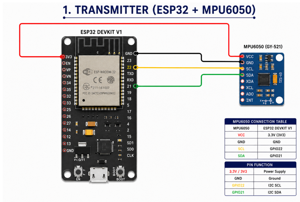
Figure 5.3: Final Transmitter Assembly
