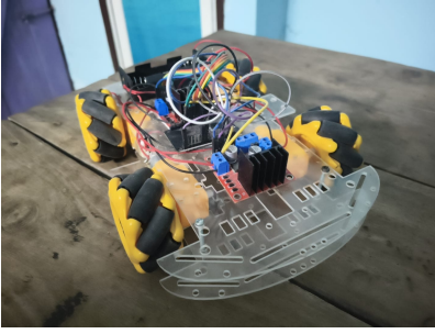
Figure 5.5: 4WD Car
