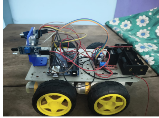
Figure 5.5: Battery Mount
