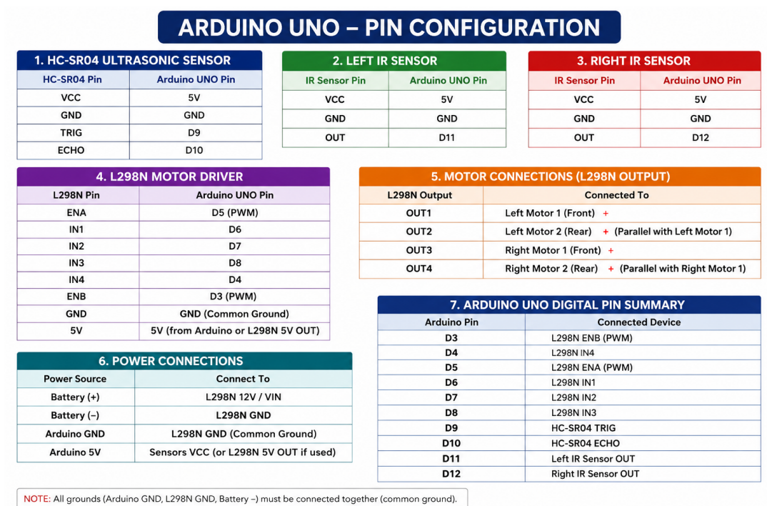
Figure 3.2: Arduino UNO and Sensor/Driver Pin Configuration Schematic
