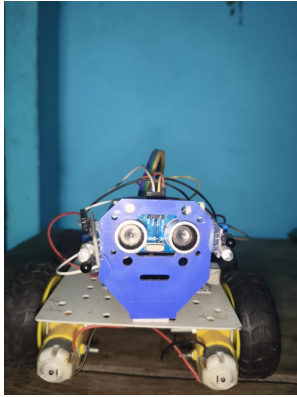
Figure 5.2: Assembled Object Following Robot
