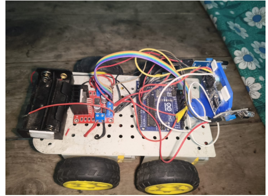
Figure 5.3: Internal Chassis Wiring and Layout
