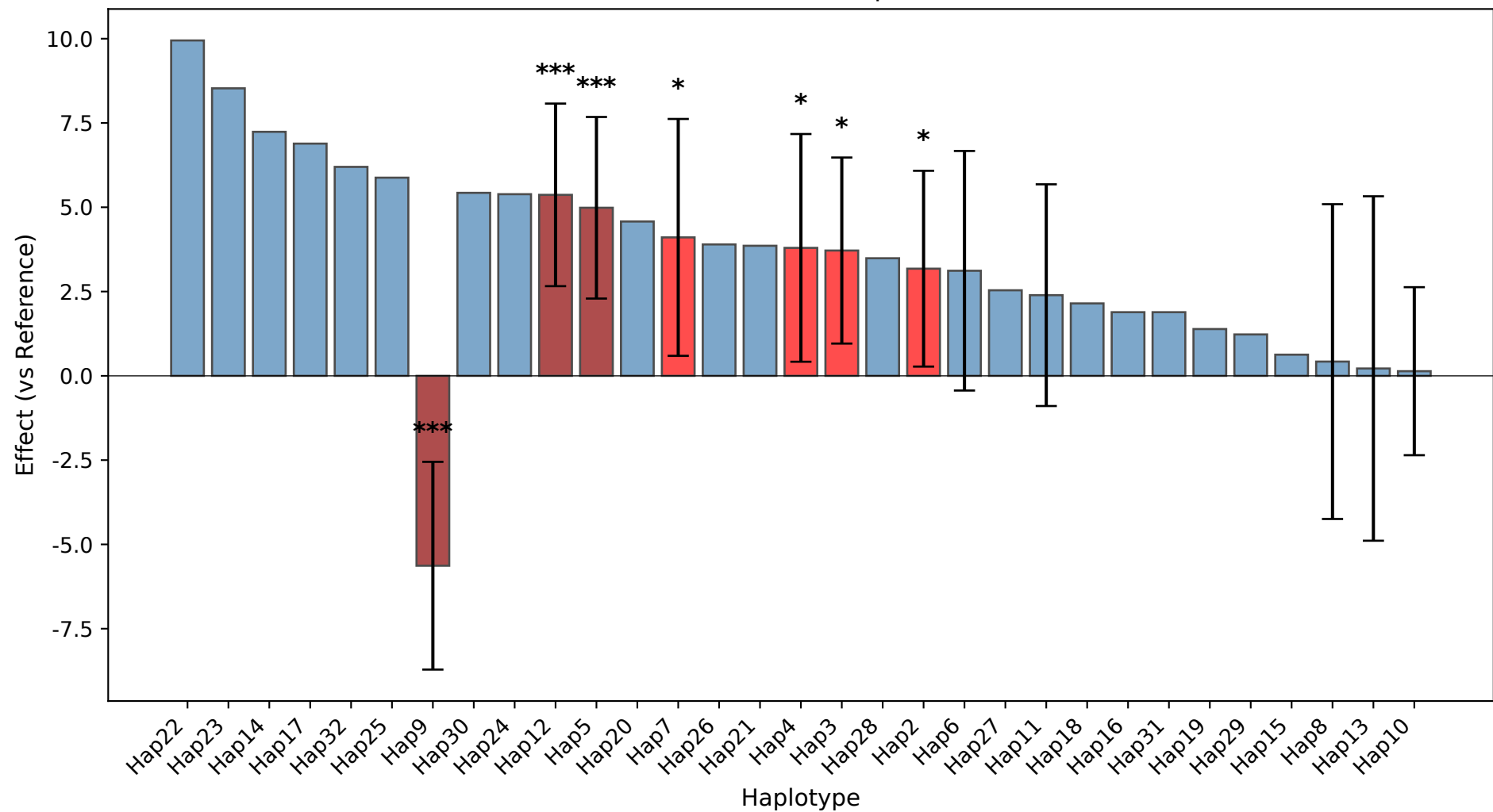
Haplotype Effects on Spikelet_length (Reference: Hap1)
