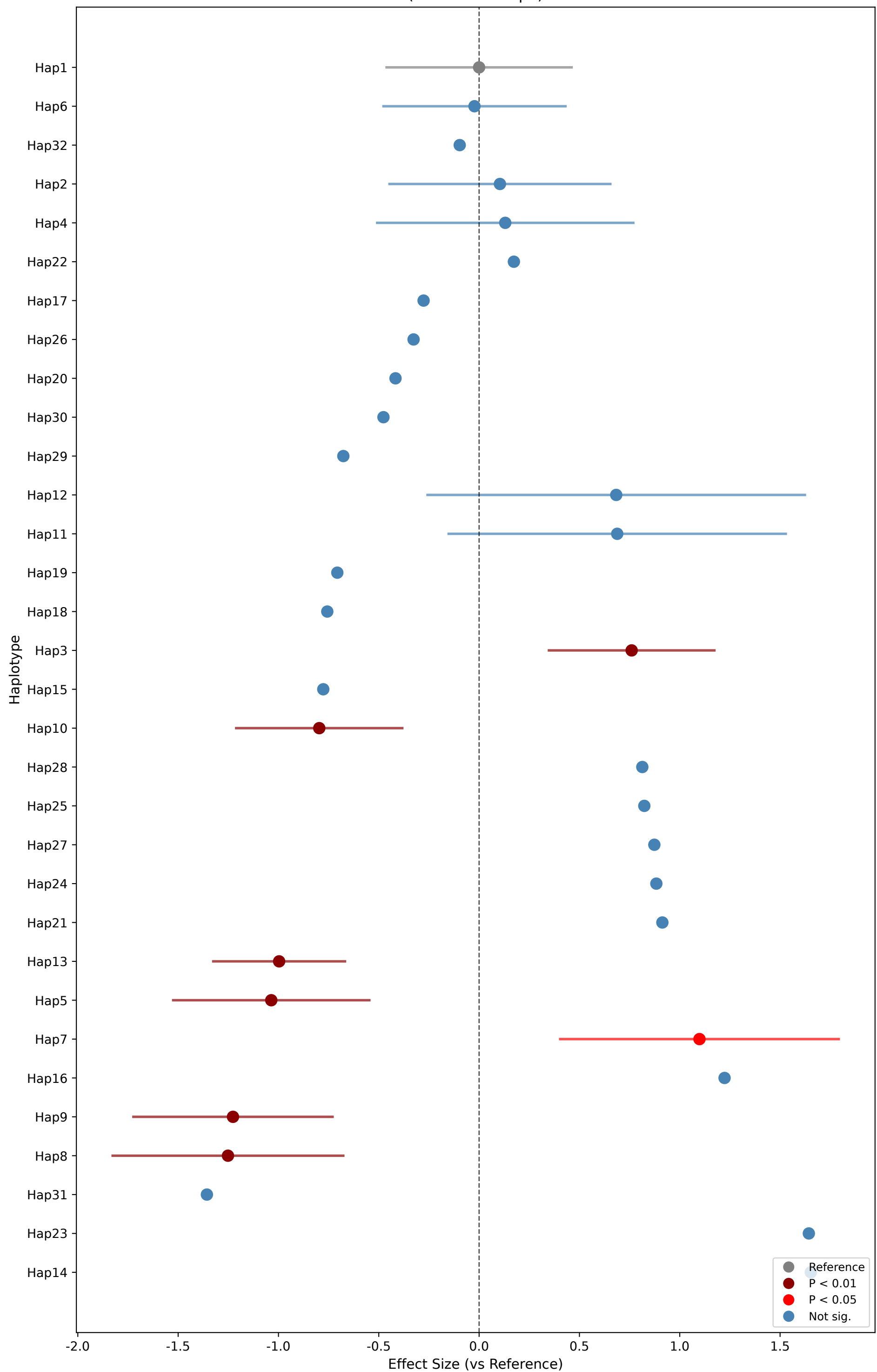
Haplotype Effect Analysis: Grain_length (Reference: Hap1)
