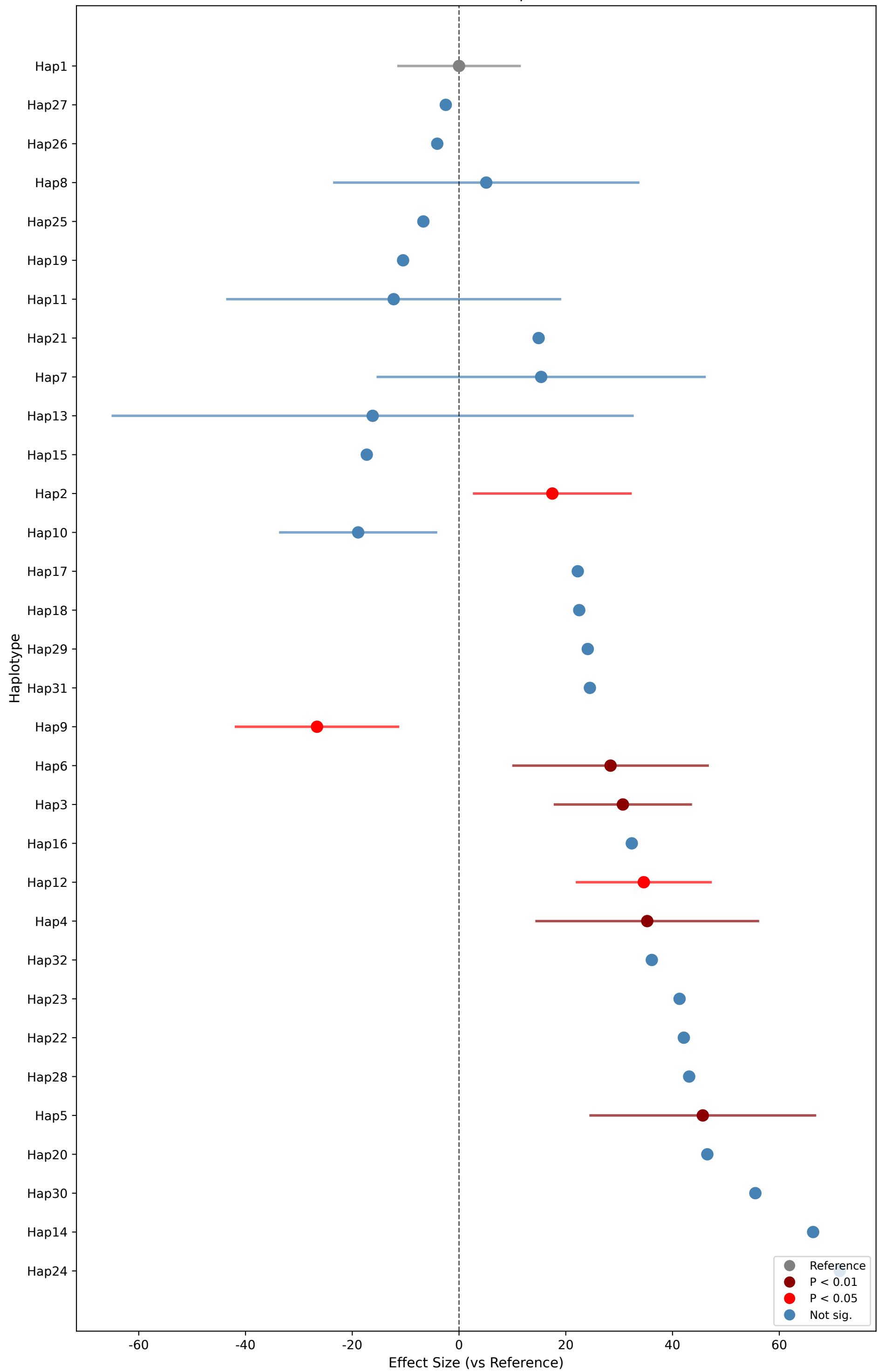
Haplotype Effect Analysis: Plant_height (Reference: Hap1)
