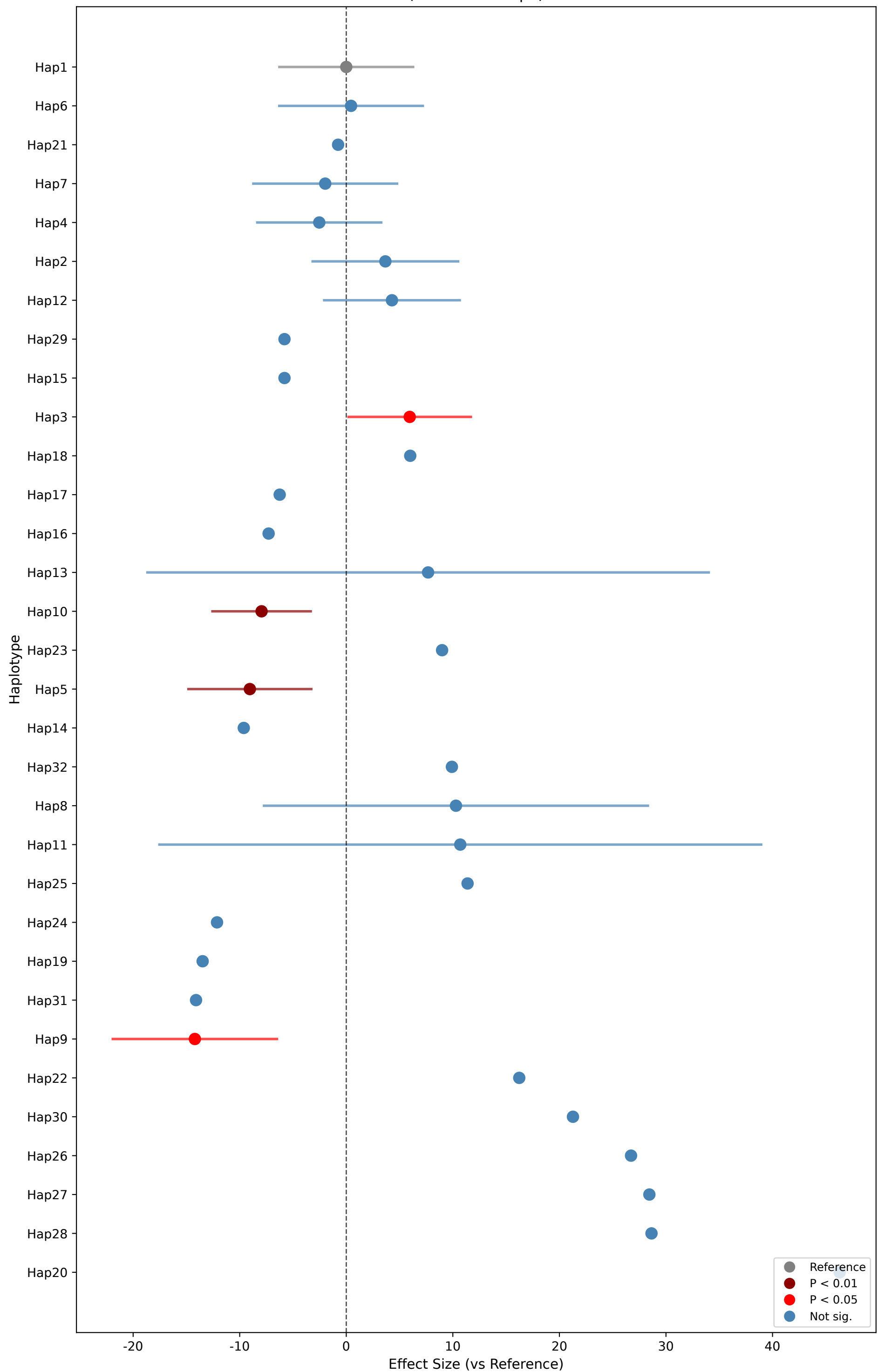
Haplotype Effect Analysis: Yield (Reference: Hap1)
