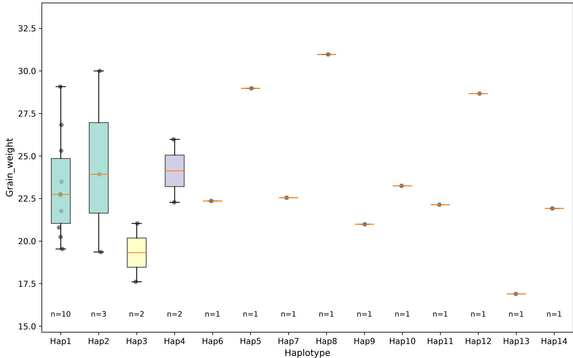
GW7 Haplotype-Phenotype Association: Grain_weight P = 0.29 ns
