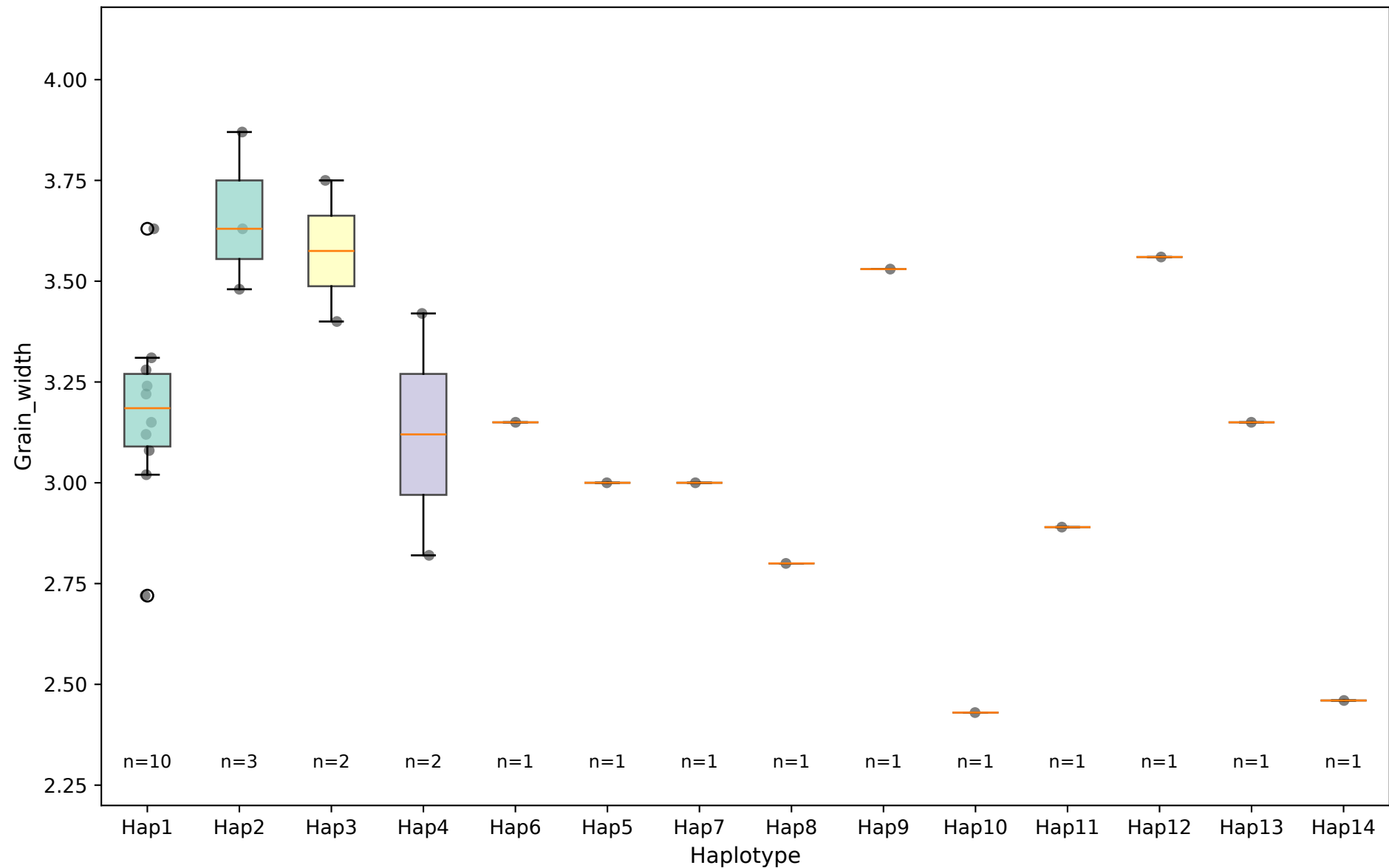
GW7 Haplotype-Phenotype Association: Grain_width P = 0.020 *
