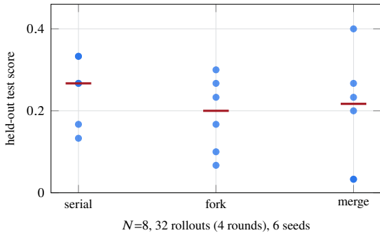
Figure 8: Fusion width 8. Per-seed test scores with medians marked. The three arms overlap; the merge arm has the widest spread (s.d. 0.130 against 0.076 and 0.085).
