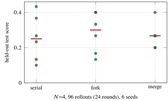
Figure 9: Fusion width 4, matched to the trust region, at a 3\times budget, six seeds. The arms still overlap, but the merge arm is the tightest (s.d. 0.067 against 0.118 and 0.105) — the ordering that width 8 reverses.
