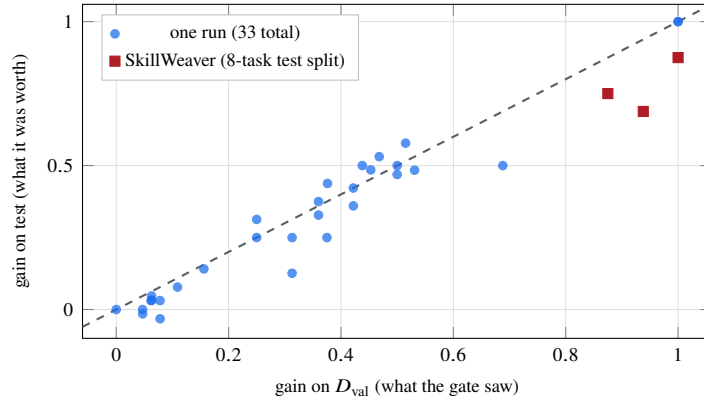
Figure 7: How optimistic the acceptance gate is, over the 33 runs of Fig. 6. Each point is one run: what its accepted diffs gained on the reused D_{\text{val}} against what they gained on a disjoint test split. Points on the dashed diagonal realized exactly what the gate measured; points below it are the adaptive-data-analysis penalty for reusing one holdout across hundreds of acceptance decisions. Twenty of 33 fall below, 7 above, 6 exactly on it (two-sided sign test on the 27 non-tied runs, p = 0.019 ), at a mean shortfall of 0.038 — roughly a tenth of the mean gain, and not enough to change the sign of any result. The three largest shortfalls are the runs with the coarsest reward signal, marked separately.
