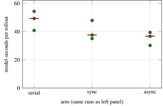
Figure 4: Validation-cost reduction in the same runs (Section 5.3): model-seconds spent per rollout at a pinned rollout budget, per seed, with medians marked. The parallel arms evaluate less per unit of work — median 49.3 \rightarrow 37.6 \rightarrow 36.7 — because reflective merge collapses each round’s admissions into one gate sweep and stale proposals are discarded before they are scored.
