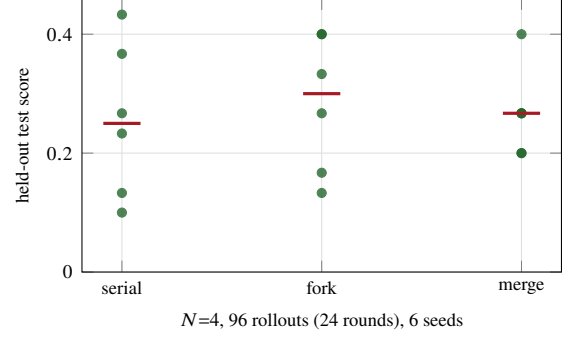
Figure 9: Fusion width 4, matched to the trust region, at a 3\times budget, six seeds. The arms still overlap, but the merge arm is the tightest (s.d. 0.067 against 0.118 and 0.105) — the ordering that width 8 reverses.
