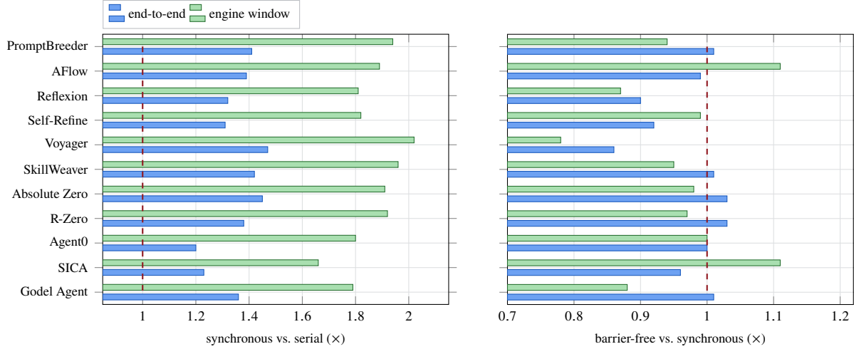
Figure 5: RQ2, per method: the two halves of the scheduler result, on the same eleven ports and the same runs. Left: synchronous parallelism against the serial control clears 1.0 (dashed) for all eleven methods on both clocks — unanimous, p = 0.001 by a two-sided sign test on each. Right: removing the barrier, against synchronous, straddles 1.0: 5 methods faster and 5 slower end-to-end ( p = 1.00 ), 2 faster and 8 slower in the engine window ( p = 0.11 ). The two panels use different x ranges and neither starts at zero, so bar lengths are not comparable across panels — read the positions against the dashed line. This is the regime distinction of Section 5.3 made visible — these compact ports have little heavy-tailed rollout latency or gate cost for asynchrony to hide, unlike the gate-heavy workload of Fig. 3.
