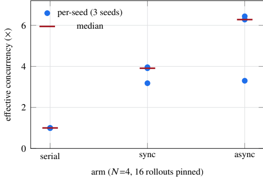
Figure 3: Effective concurrency (model-seconds \div wall-clock), GEPA on HotpotQA, GLM-5.2, 16 rollouts pinned per arm, three seeds. The serial control reproduces the published loop (one worker, serial gate) and lands at 0.99–1.00 \times on every seed — the control property is a stable one, not a single-run coincidence. Synchronous parallelism spans 3.18–3.96 \times ; barrier removal spans 3.30–6.44 \times but is by far the widest arm, and it reaches those figures while overrunning the pinned budget (19 rollouts against 16).
