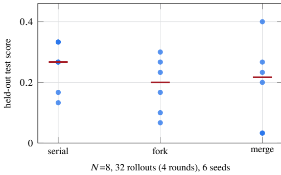
Figure 8: Fusion width 8. Per-seed test scores with medians marked. The three arms overlap; the merge arm has the widest spread (s.d. 0.142 against 0.084 and 0.093).
