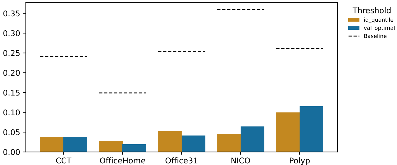
Accuracy-prediction MAE
